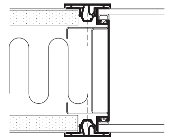
Gypsum board joint type 1290
