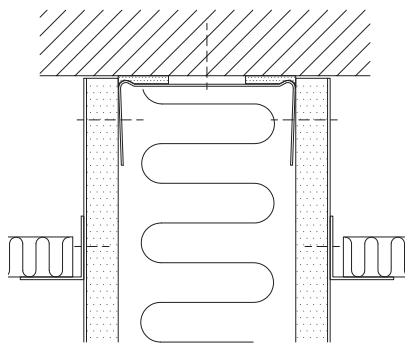
Suspended ceiling connction
