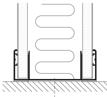
Floor connection
