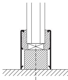
Floor connection
