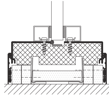
Floor connection
