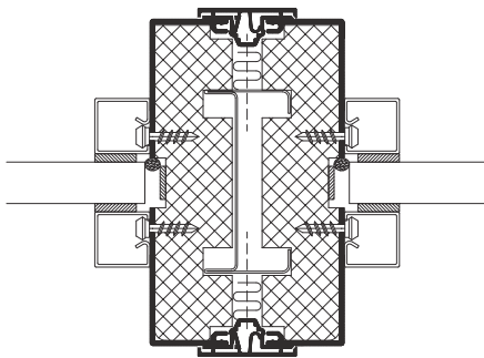
Glass joint - single glazed
